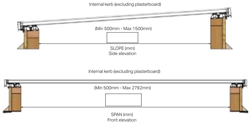
Spans up to 2792mm and slopes of 1500mm – see matrix for configuration details.
